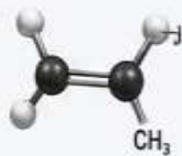
Propylene (from which Polypropylene is made)
