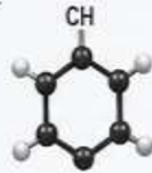
Styrene (from which Polystyrene is made)
